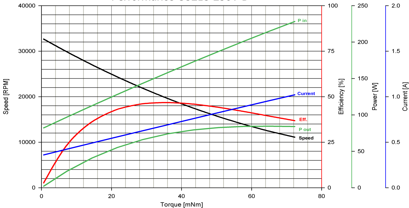
Performance U5215 230V D
