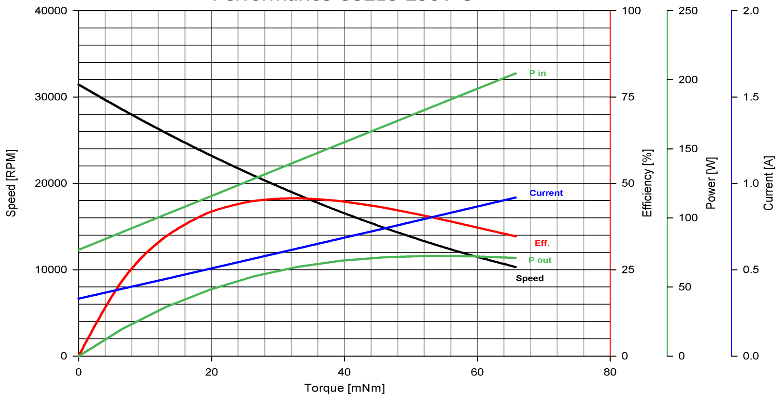
Performance U5215 230V C
