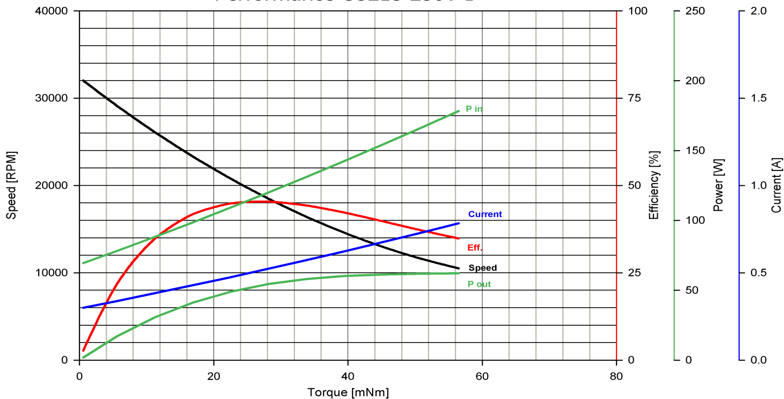
Performance U5215 230V B
