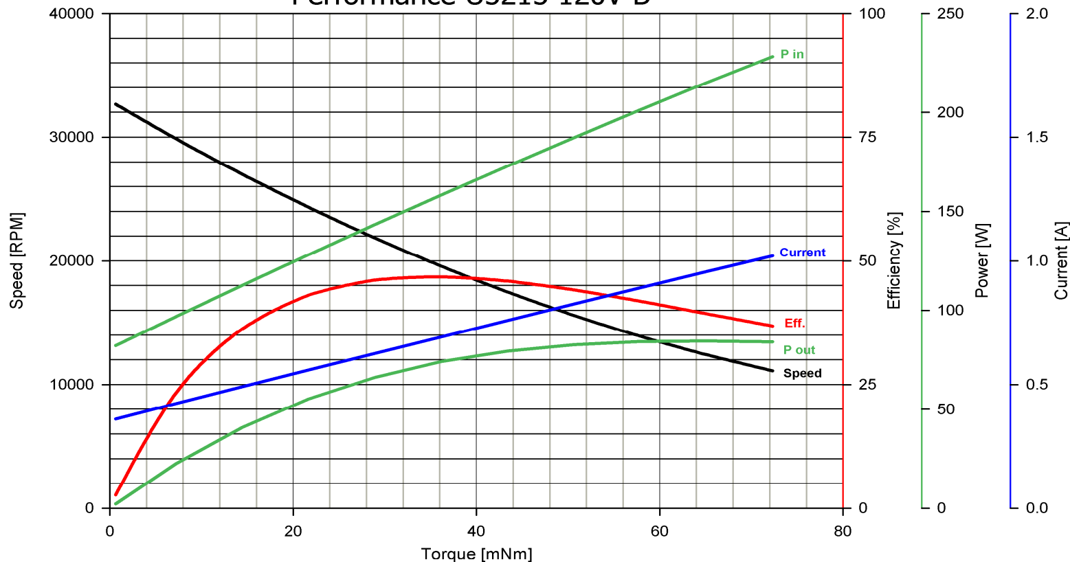
Performance U5215 120V B
